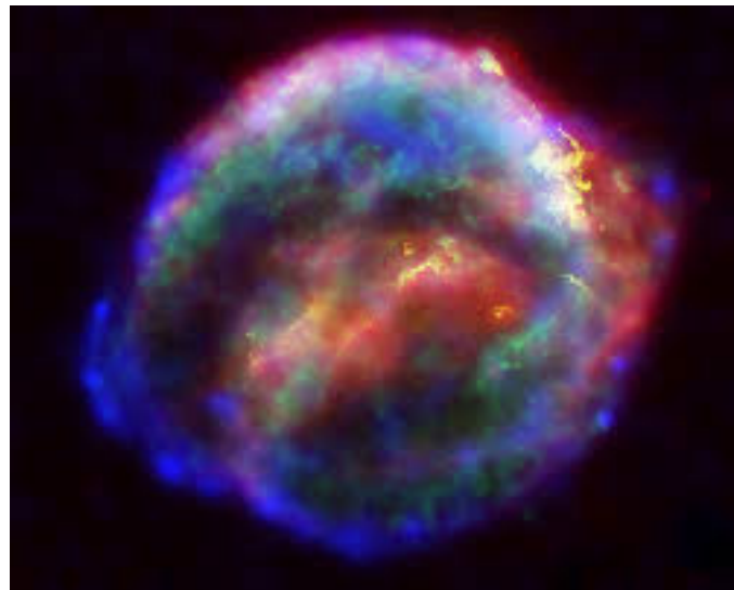
Star explosion (Supernova)
